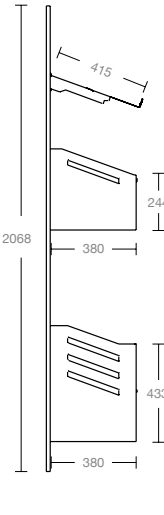
RETRO PANETTERIA BACK BAKERY UNIT
