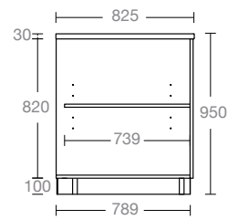
BANCO NEUTRO H950 P825MM AMBIENT COUNTER H950 P825MM
