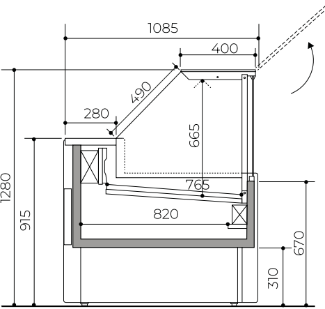
FREDDO STATICO CON CELLA STATIC COLD WITH REFRIGERATED STORAGE Dim: 1500-2000-2500-3000 mm
