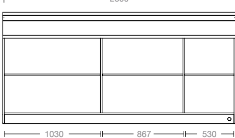
BANCO BAR NEUTRO L2500 H1200 P905MM AMBIENT BAR COUNTER W2500 H1200 P905MM
