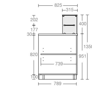
BANCO NEUTRO CON CASTELLO VETRI H1350 P825 MM AMBIENT COUNTER WITH FRAME GLASS H1350 D825 MM
