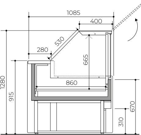
CALDO SECCO _ DRY HEATED Dim: 1000-1500 m
