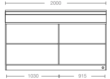
BANCO BAR NEUTRO L2000 H1200 P905MM AMBIENT BAR COUNTER W2000 H1200 P905MM
