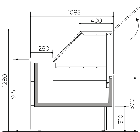
BAGNOMARIA _ BAIN MARIE Dim: 1500 mm
