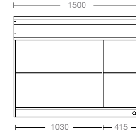
BANCO BAR NEUTRO L1500 H1200 P905MM AMBIENT BAR COUNTER W1500 H1200 P905MM
