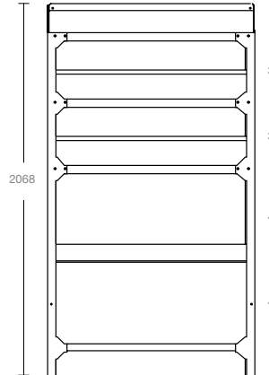
SCAFFALE PANETTERIA A TERRA 1000 P 383 HIGH BAKERY SHELF UNIT 1000 D 383
