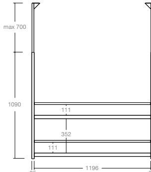
MENSOLA PORTA BOTTIGLIE A SOFFITTO CEILING BOTTLE COMPARTMENT
