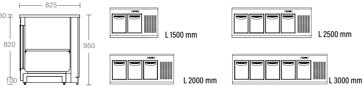
BANCO CON CELLE REFRIGERATE STATICHE E MOTORE INCORPORATO H950 P825 MM COUNTER WITH STATIC REFRIGERATED ROOMS & HERMETIC UNIT H950 D825 MM
