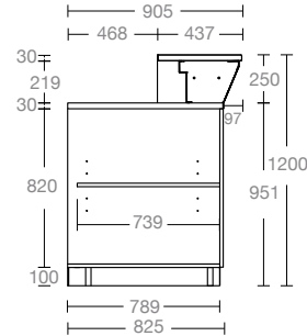
BANCO BAR NEUTRO H1200 P905MM AMBIENT BAR COUNTER H1200 P905MM
