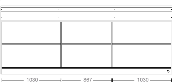
BANCO BAR NEUTRO L3000 H1200 P905MM AMBIENT BAR COUNTER W3000 H1200 P905MM
