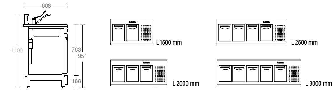
BASE CON CELLE REFRIGERATE STATICHE E MOTORE INCORPORATO H1100 P668 MM BACK-BASE WITH STATIC REFRIGERATED ROOMS & HERMETIC UNIT H1100 D668
