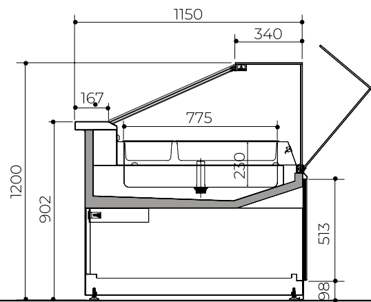
BAGNOMARIA _ BAIN MARIE Dim: 1500 mm
