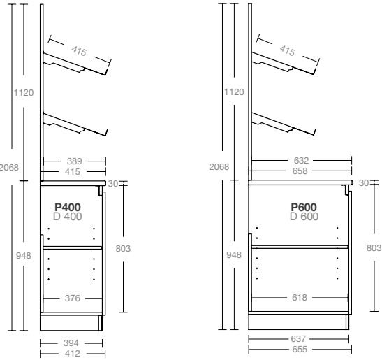
ALZATA BASE RETRO CON PIANI PORTACESTI INCLINATI WALL-MOUNTED UNIT AND BAR-BACK BASE UNIT WITH TILTED SHELVES
