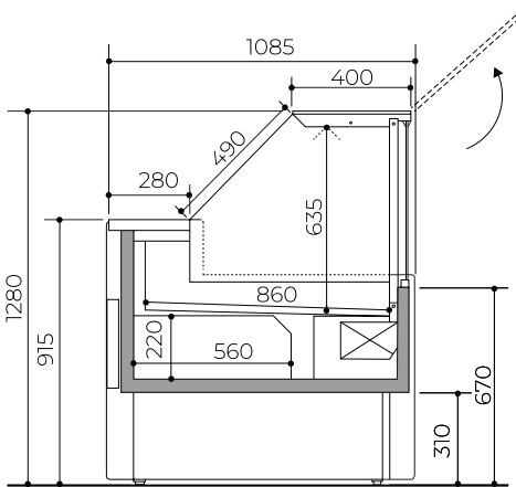
FREDDO VENTILATO CON CELLA VENTILATED COLD WITH REFRIGERATED STORAGE Dim: 1500-2000-2500-3000 mm
